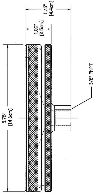
ASSEMBLY VIEW OF FJ-110mm
